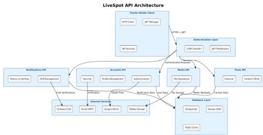
Figure 4.6: LiveSpot REST API Architecture - Vertical layout showing layered architecture from Flutter client through authentication middleware to organized API endpoints with external service integrations
