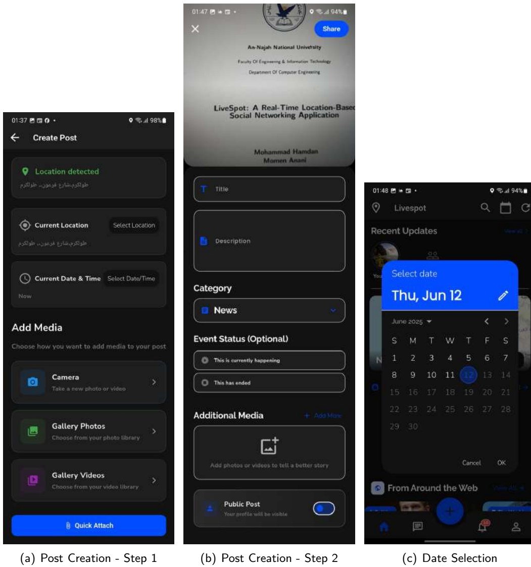
Figure 5.11: Content Creation Flow on Android—Multi-Step Post Publishing
