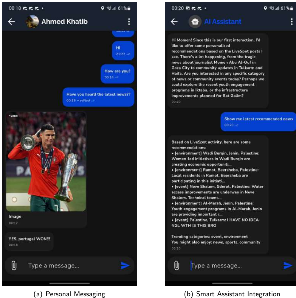
Figure 5.13: Messaging System on Android—Communication and Smart Assistant Features
