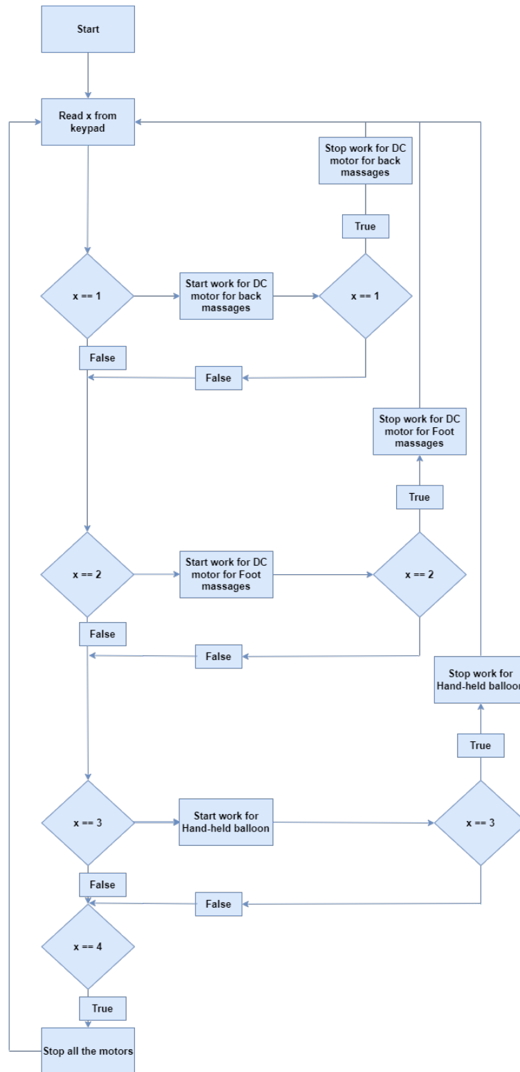
Figure 4.23: Full diagram
