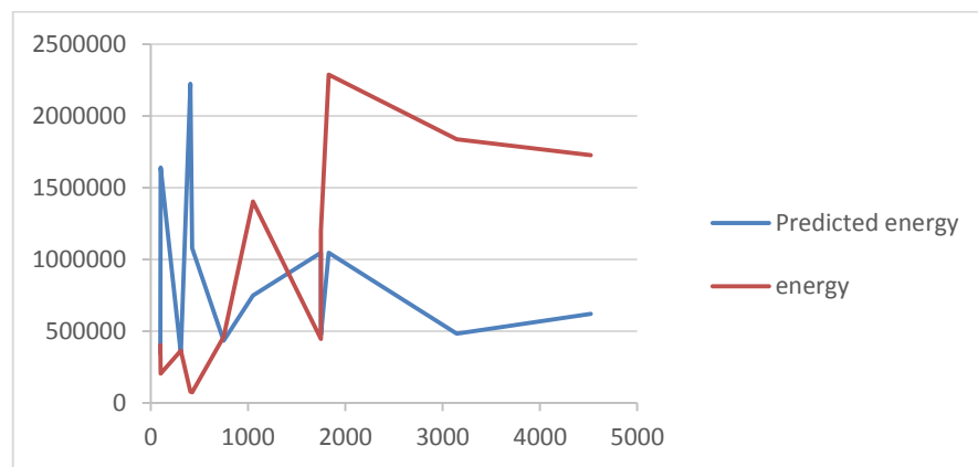
Figure 22: The relationship between: Predicted Energy kj VS Real measures kj
