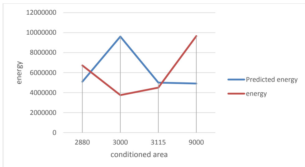
Figure 15: Predicted Energy kj VS Real measures kj.
