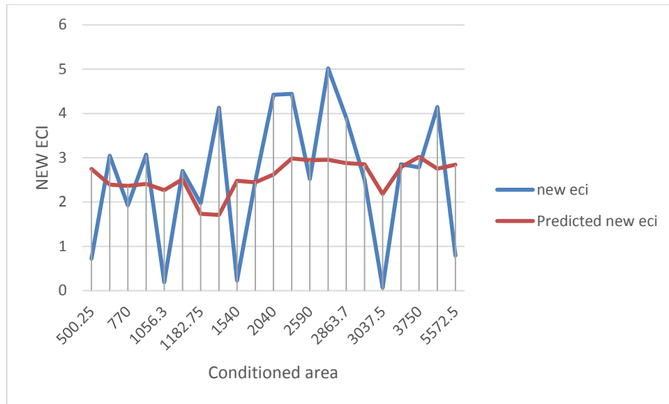
Figure 27: Predicted ECI \text{nis/m}^2 VS Real measures
