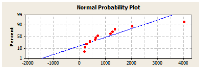
Figure 16: Normal Probability plot for Restaurants and Hotels EUI.
