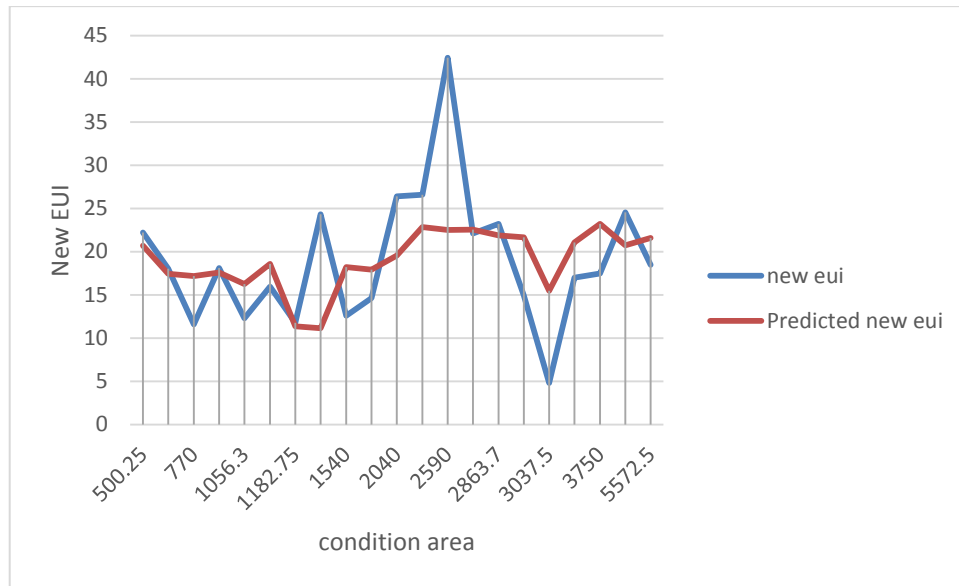
Figure 24: Predicted EUI VS Real measures
