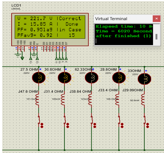
Figure 27: PF.avg a period of time of 100 minutes
