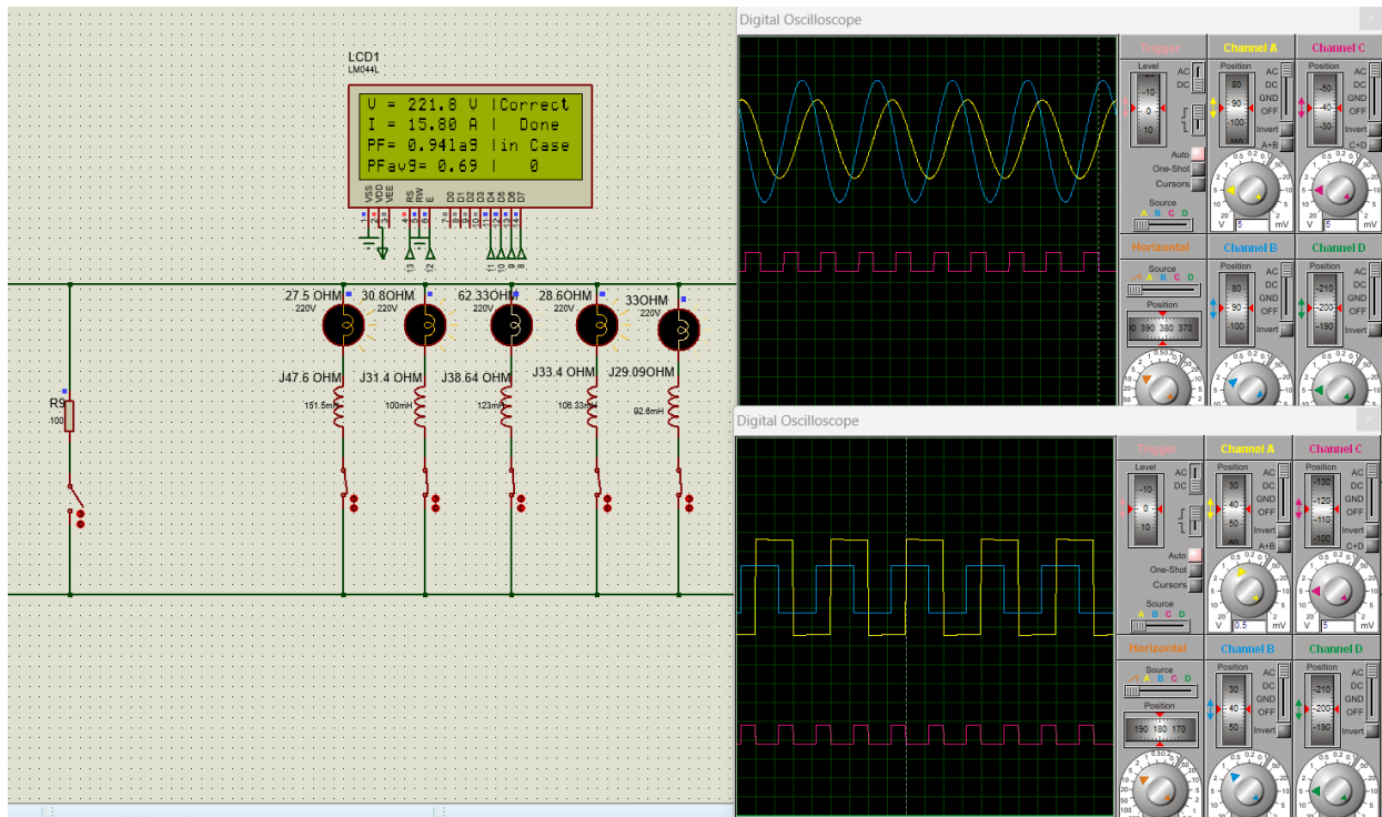
Figure 31: Waveforms with five loads on and capacitors activated.
