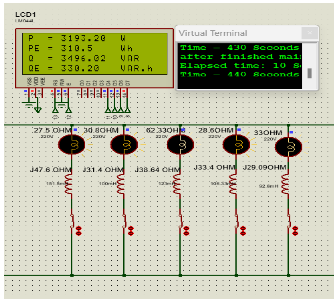
Figure 23: Real energy and reactive energy before activating the capacitor bank for case 6
