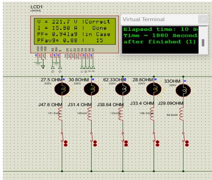
Figure 26: PF_{avg} a period of time of 30 minutes
