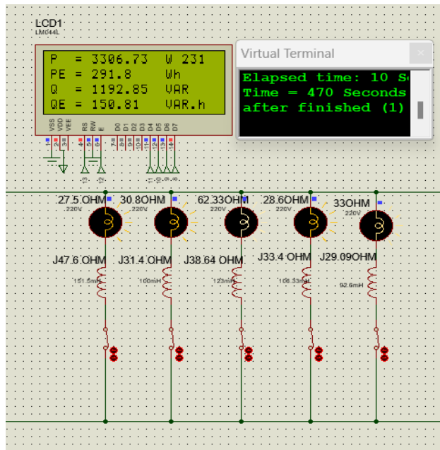
Figure 25: Real energy and reactive energy after activating the capacitor bank for case 6
