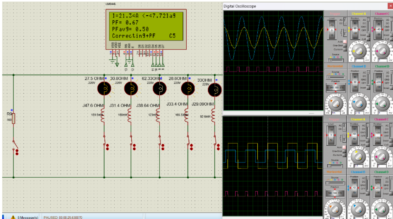
Figure 30: Waveforms with five loads running and capacitors disconnected.
