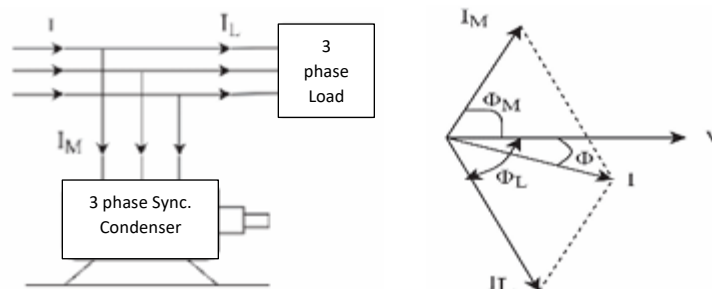
Figure 2: power factor correction using Synchronous condenser.
