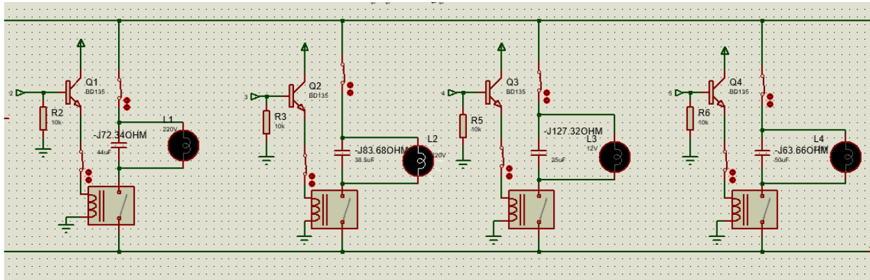
Figure 17: Capacitor Units.
