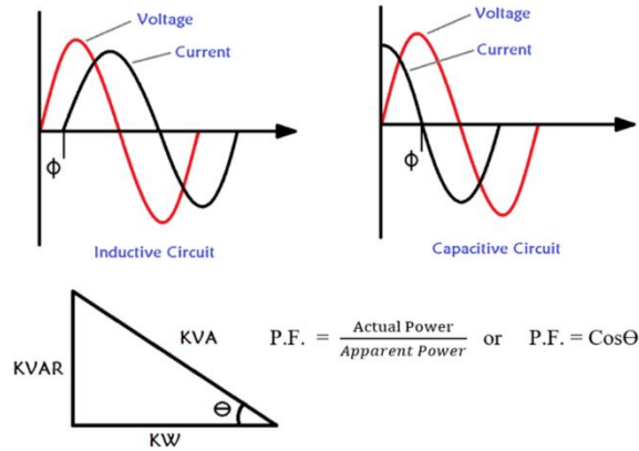
Figure 8: phase shift, and power triangle.
