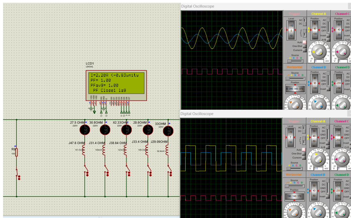
Figure 29: Waveforms with 100-ohm operation.
