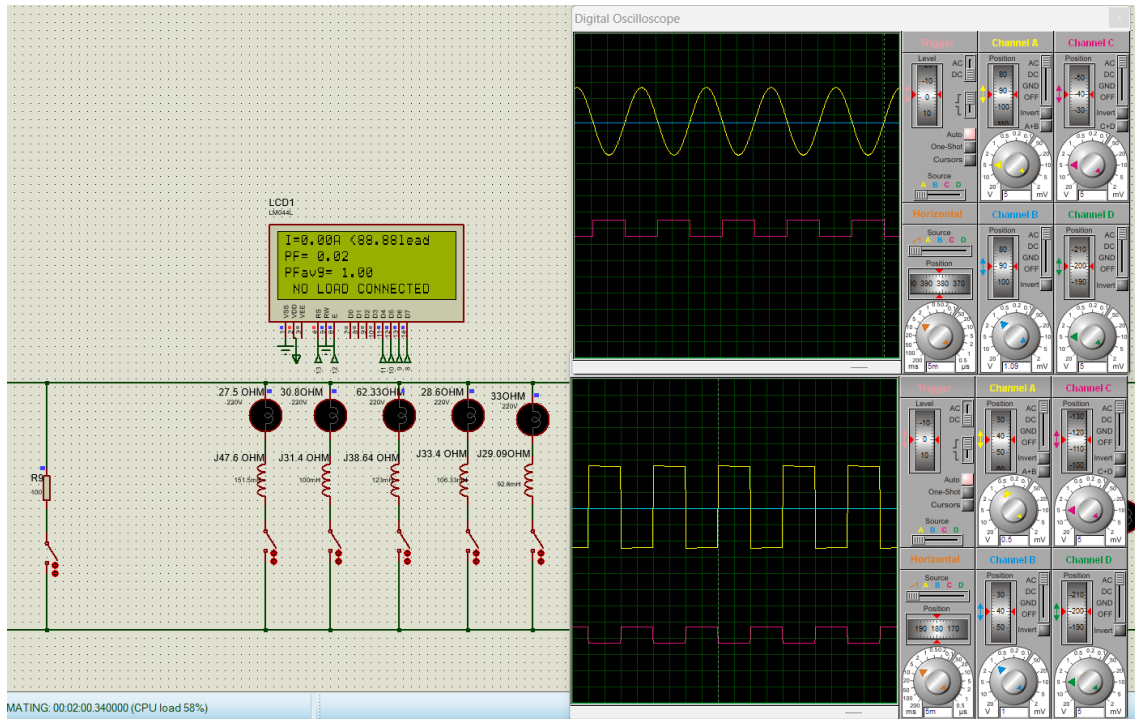
Figure 28: Waveforms with all loads separated.
