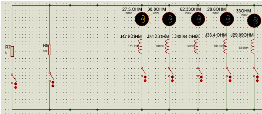
Figure 15: Load units.
