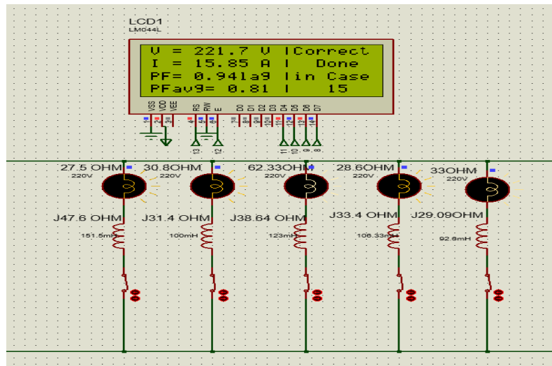
Figure 21: Phase shift value and power factor after the Correction process at case 6
