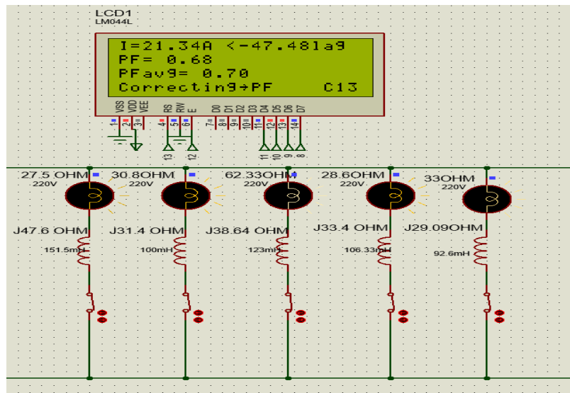
Figure 20: Phase shift value and power factor before the optimization process at case 6
