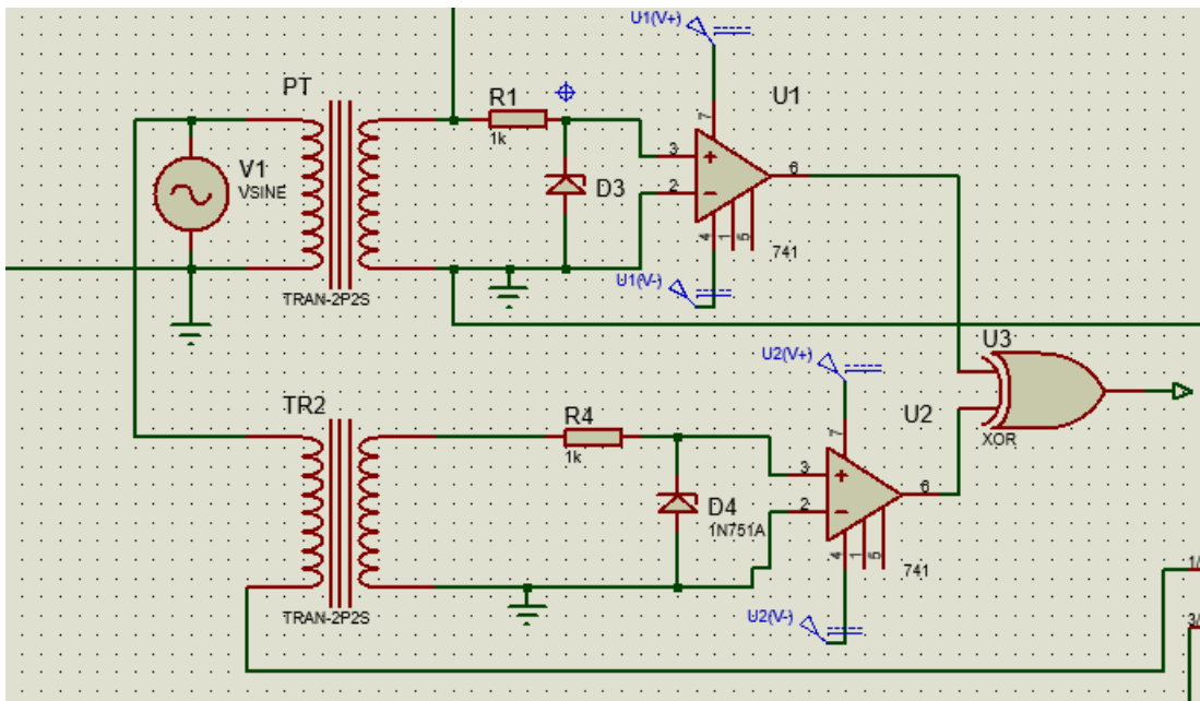
Figure 16: Phase shift display circle
