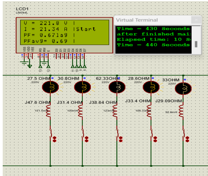
Figure 22: Value the current, power factor, and voltage before setting the capacitor bank to case 6
