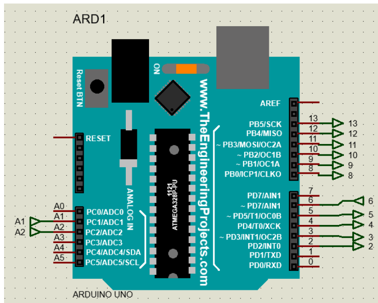
Figure 19: Arduino circuit.
