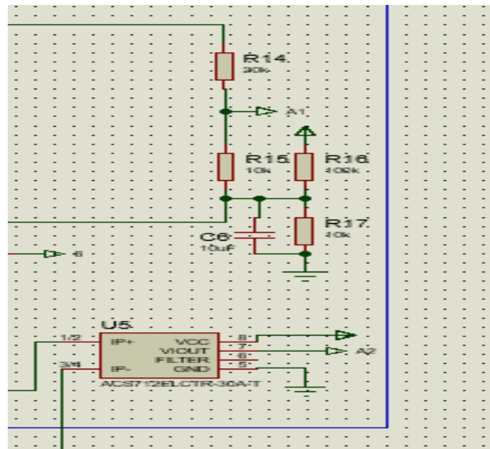
Figure 18: Current and voltage measurement circuit.
