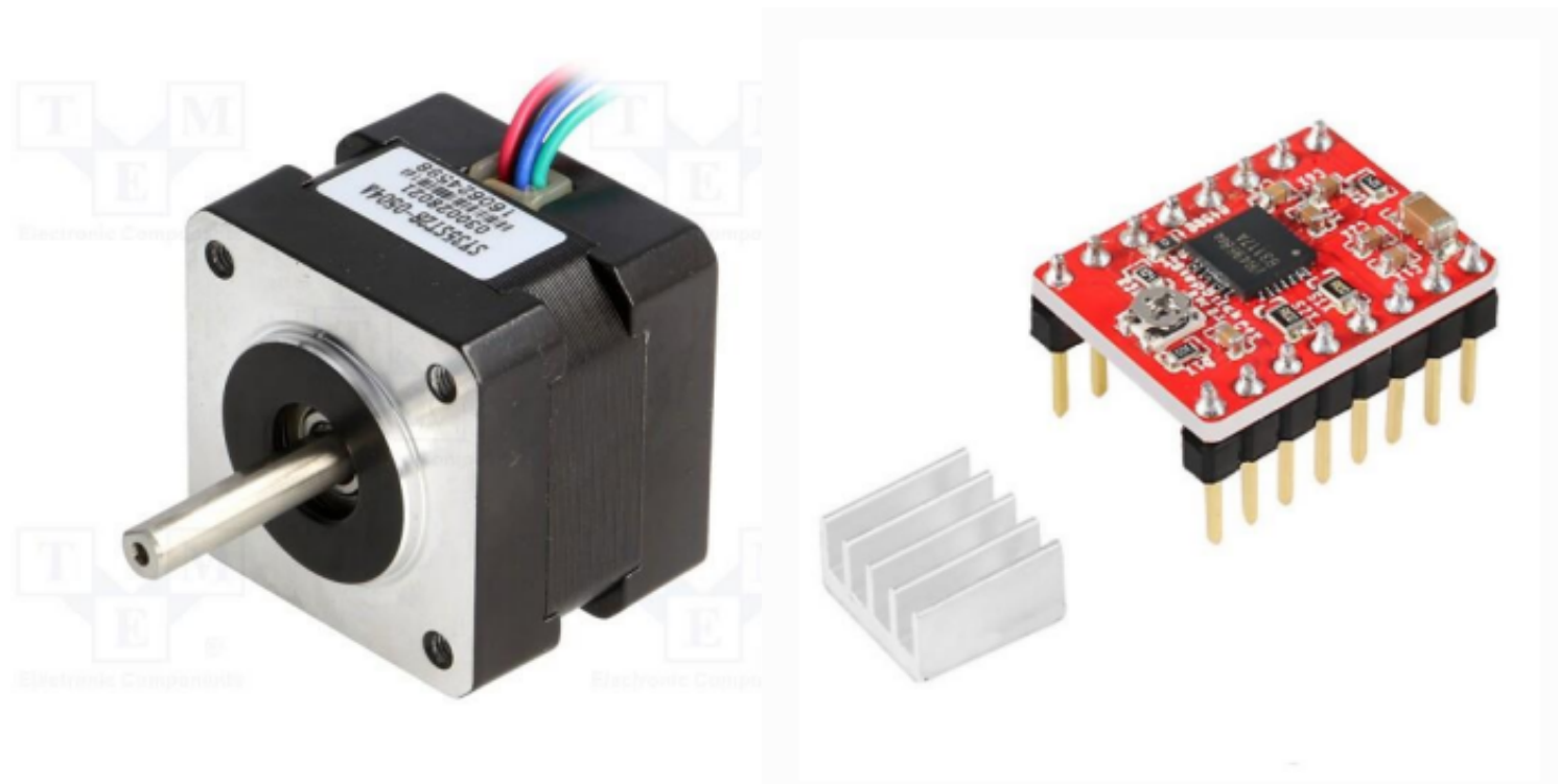
Stepper motor and A4988 Driver
