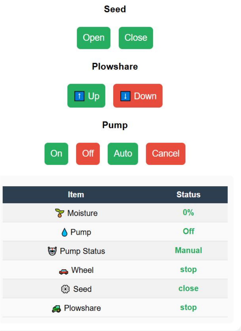
Figure 19: Interface displays the status of system
