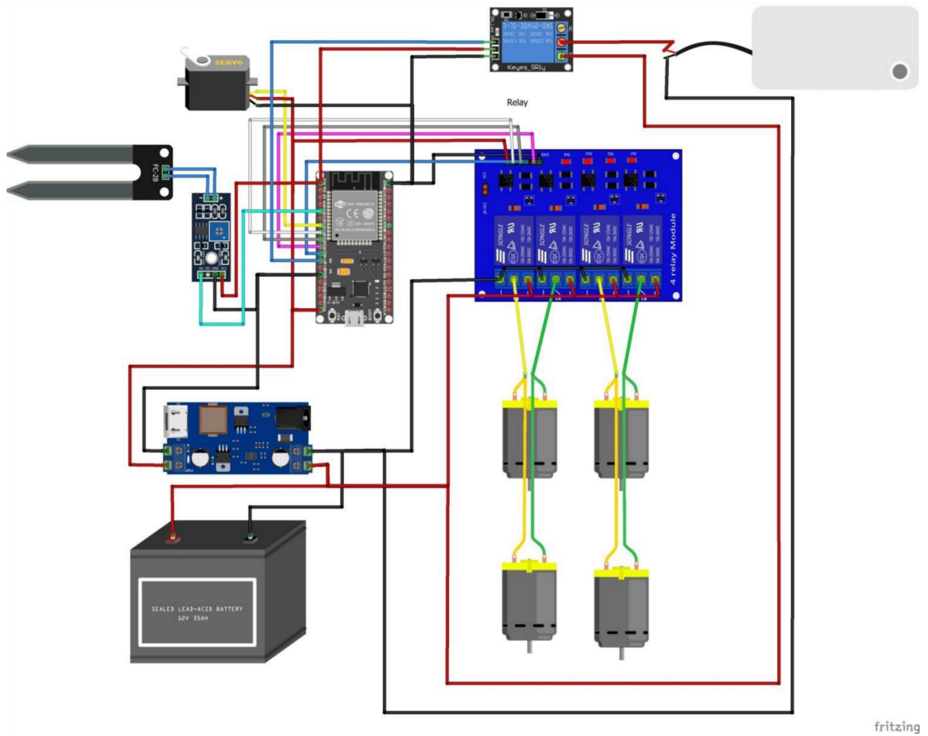
Figure 14: Wiring Diagrams
