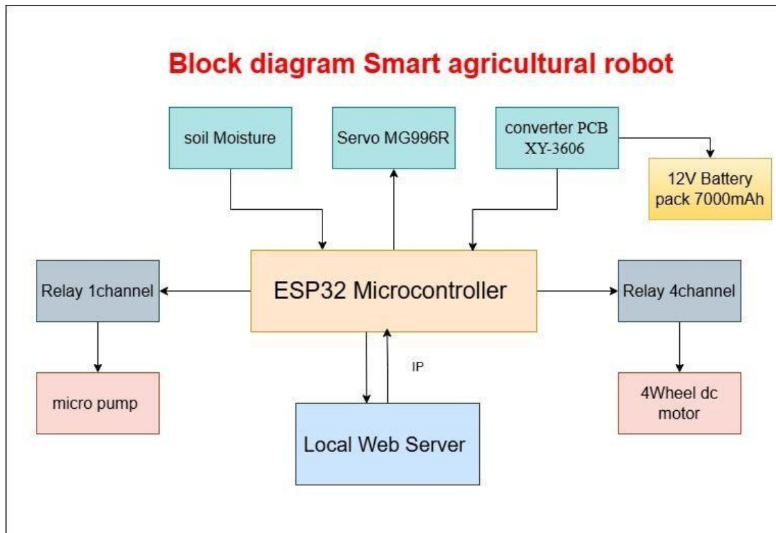
Figure 12: Block diagram
