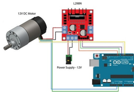
Figure 11: DC motor
