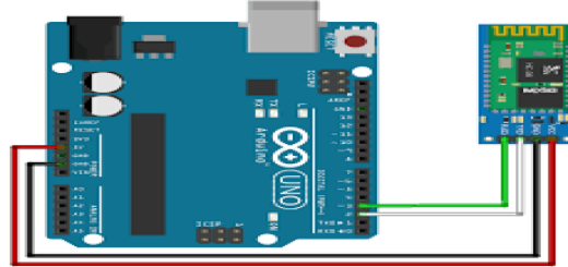
Figure 13: HC_05 Bluetooth
