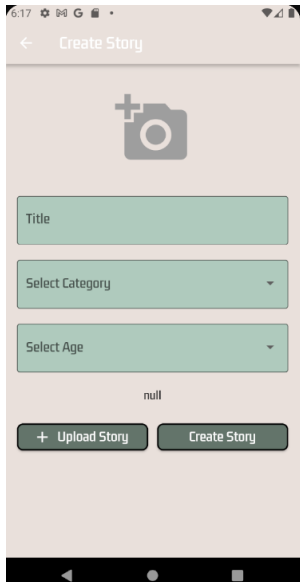
Create story
