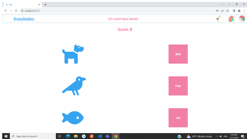
Figure 5.61: Games
