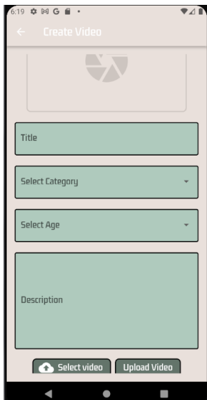
Create video
