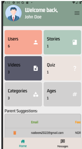
Admin sign-in
