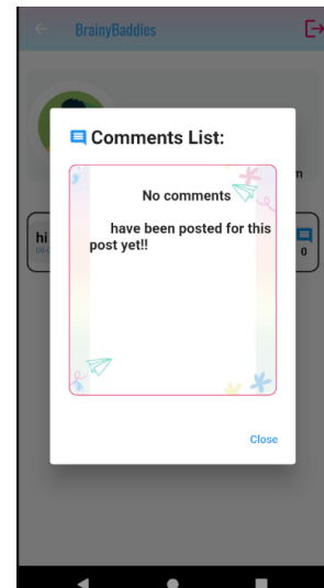
Comments List
