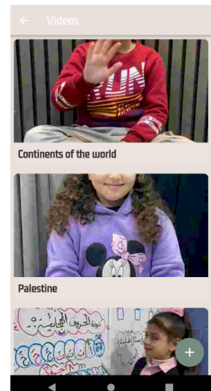
Show videos
