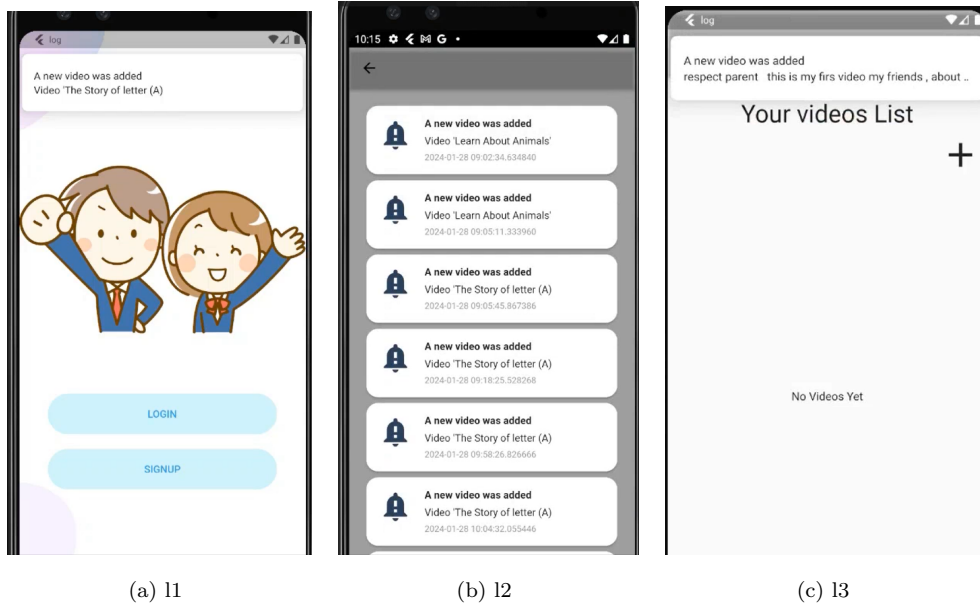
Figure 5.49: Notifications
