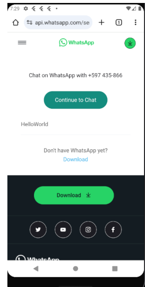
WhatsApp
