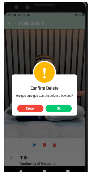
Delete Video
