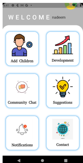
Parent Dashboard
