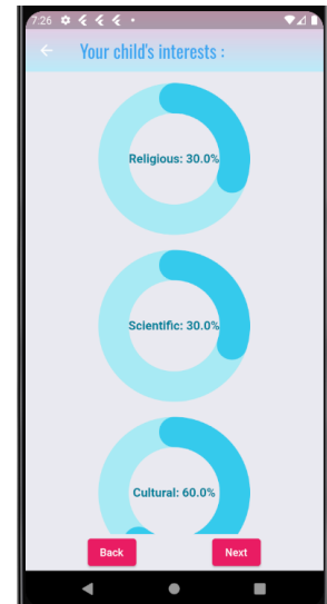
Child interests
