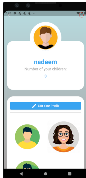
Parent Profile
