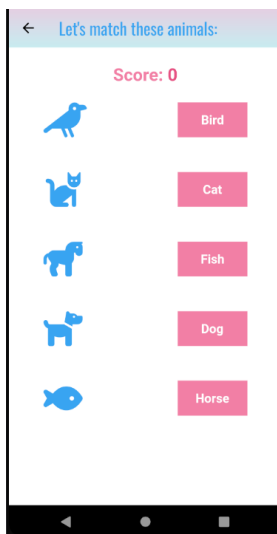
Admin Games
