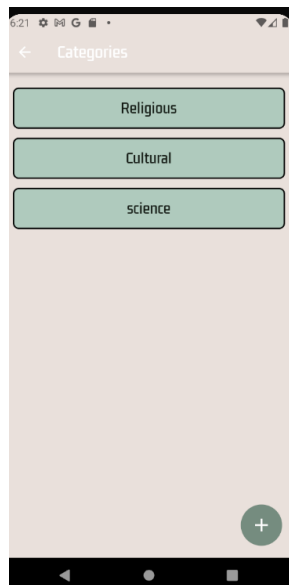
Create category
