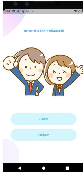
Welcome page
