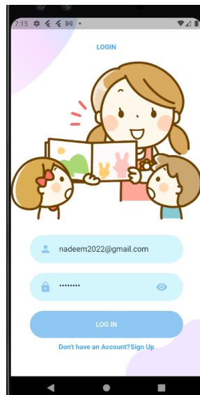
Parent Sign-in
