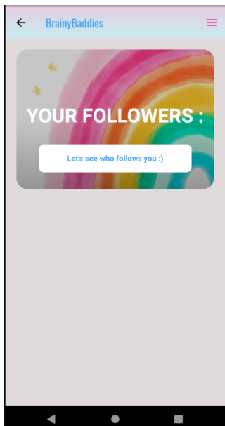
Followers List
