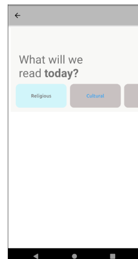
Stories categories
