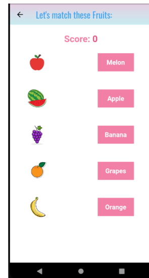
Admin Games
