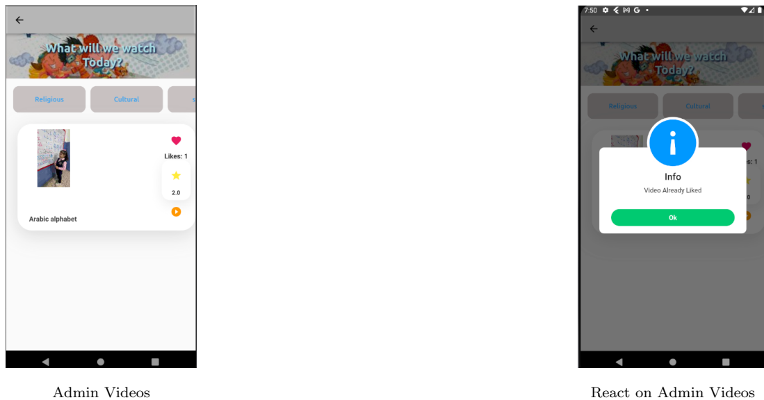
Figure 5.40: Admin Videos
