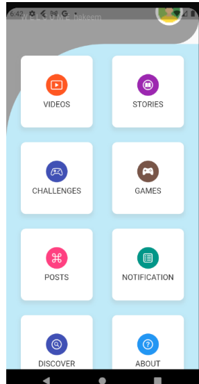
Child dashboard
