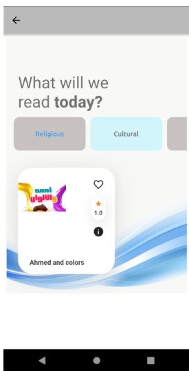
Admin Stories
