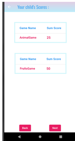
Games Scores
