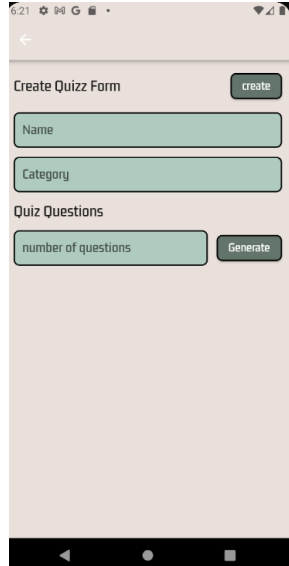
Questions
