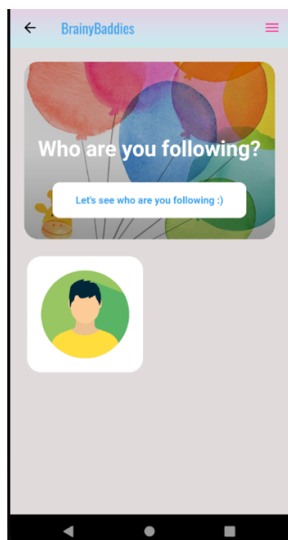
Following List
