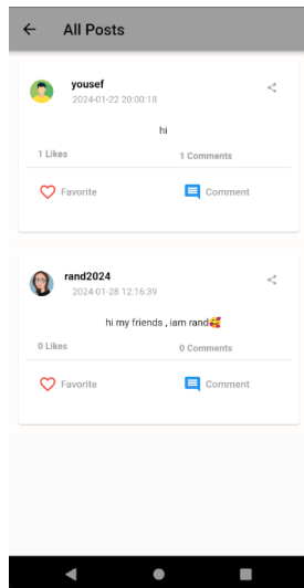
Posts List
