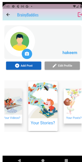
Child profile
