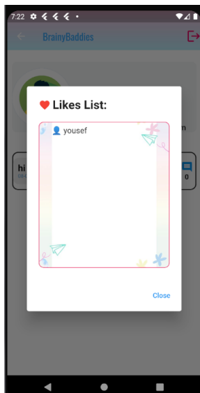
Likes List
