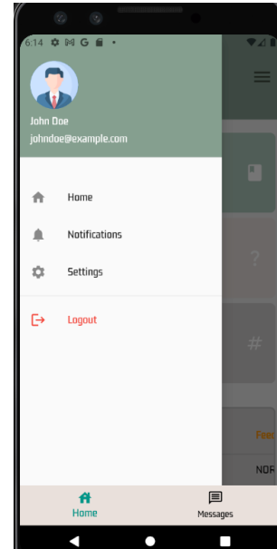
Admin Dashboard
