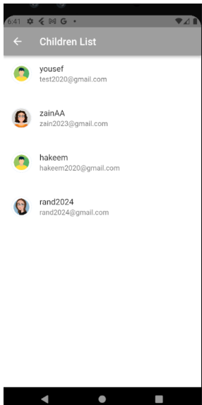
Child development
