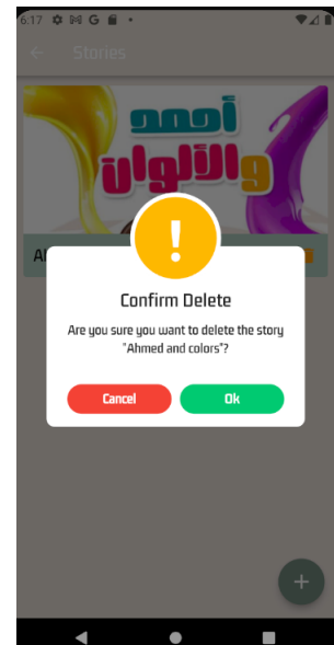
Delete Story
