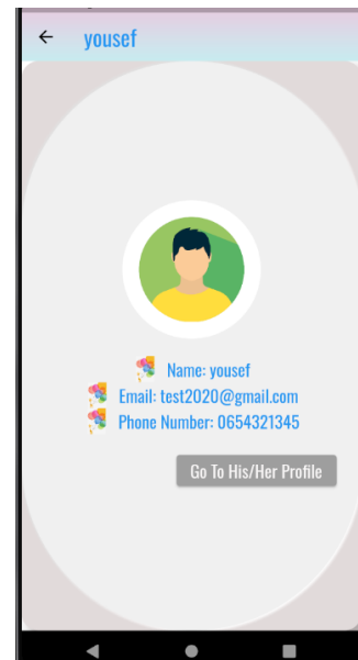
followed details
