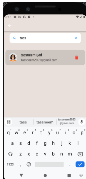
search Users
