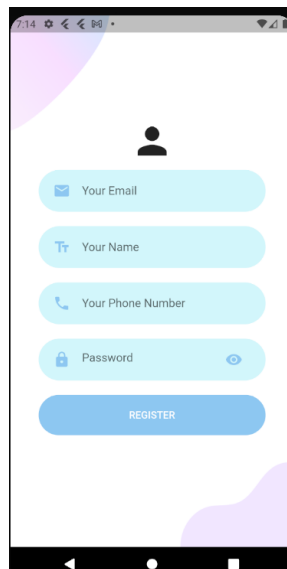
Parent Sign-up
