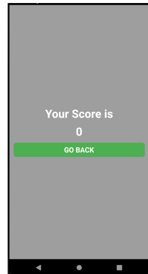
Quizzes scores
