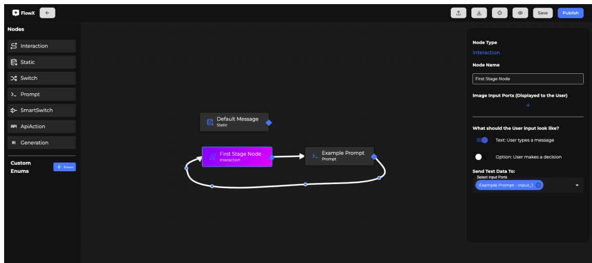
Figure 4.3: Initial Default Workflow State
