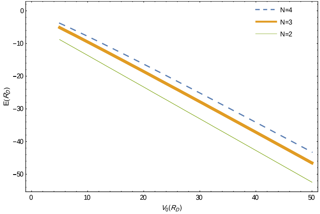
Figure (3- 4): Ground state donor energy E(1,0) as function of potential well depth ( V_0 ) and R = 2a_D for different values of dimension = 2D, 3D, 4D .
