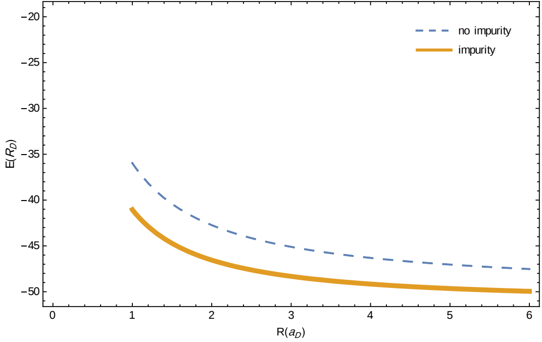
Figure 3- 1: Ground state energy E(1,0) in QD as function of dot radius ( R ) for V_0 = 50R_D, N = 3D with impurity and without impurity.
