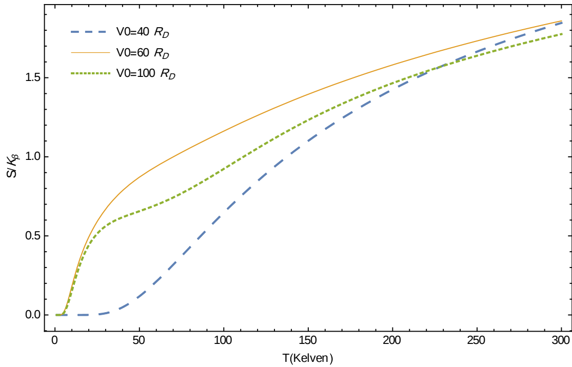
Figure (3-14) : Entropy of donor impurity in QD ( S/K_\beta ) as function of temperature ( T ) for different values of V_0 = 40R_D, 60R_D, 100R_D at constant R = 2.5a_D, N = 3D .
