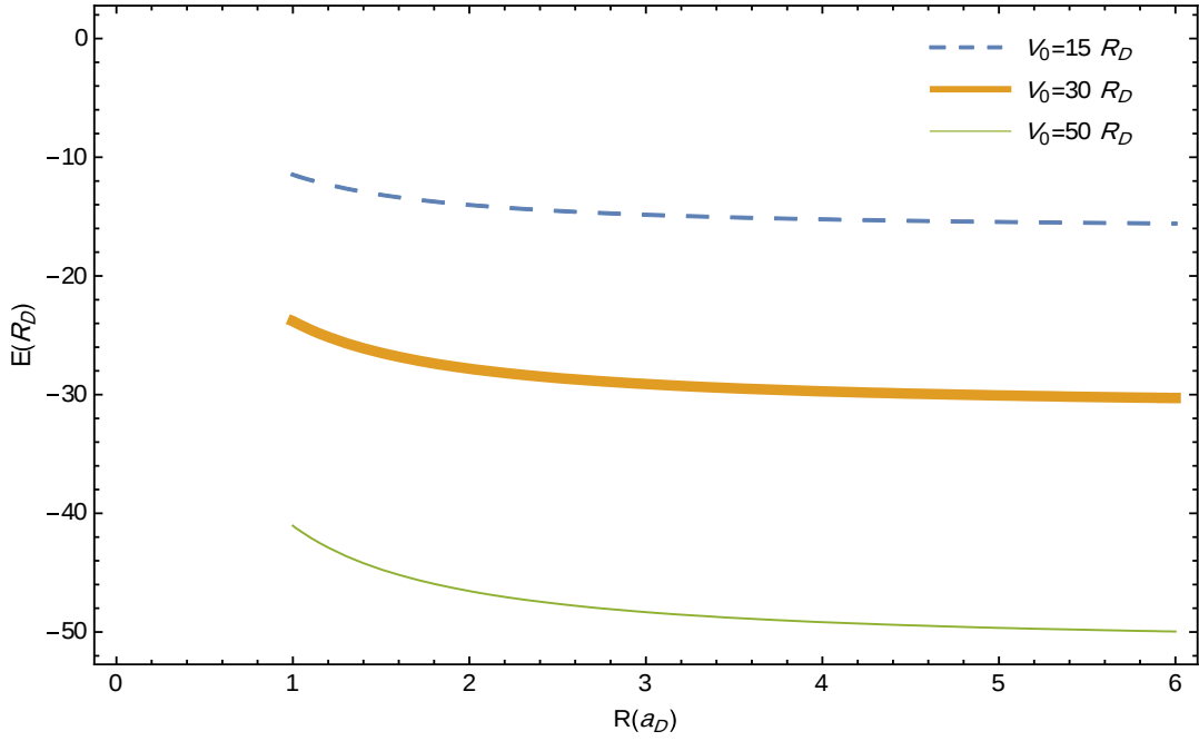
Figure (3-2): Ground state energy levels E(1,0) in QD as function of dot radius ( R ) for different values of V_0 = 15R_D, 30R_D, 50R_D , N = 3D .
