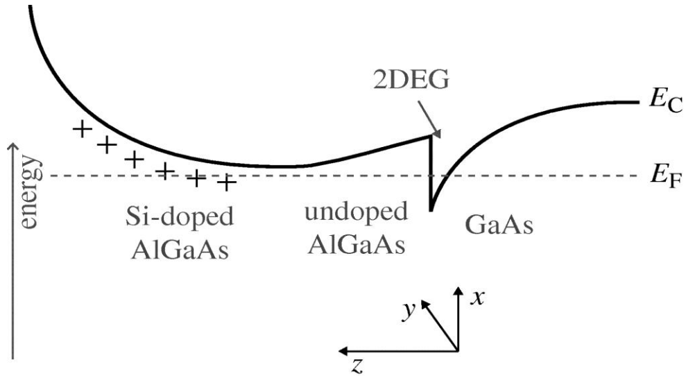
Figure (1-4 ): A sketch of forming 2DEG.
