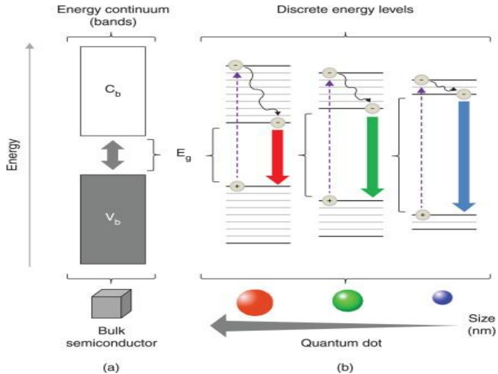
Figure (1-2): Controlling the band gap by quantum dots size.
