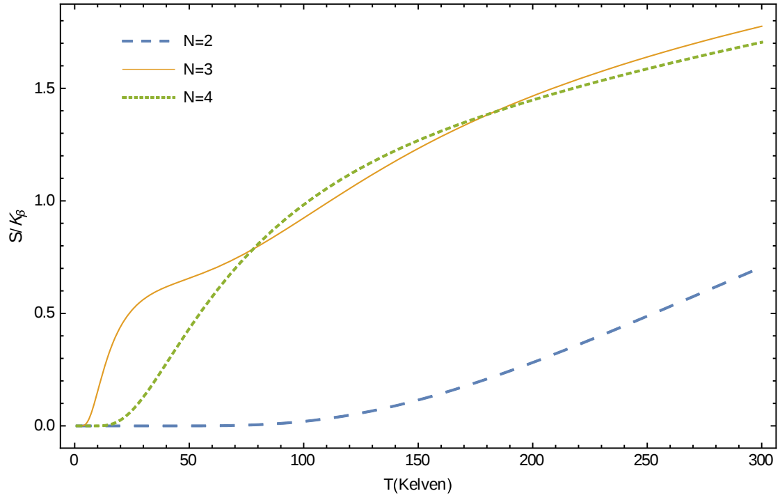
Figure (3-15): Entropy of donor impurity in QD ( S/K_\beta ) as function of temperature ( T ) for different values of N = 2D, 3D, 4D at constant R = 2.5a_D , V_0 = 100R_D .
