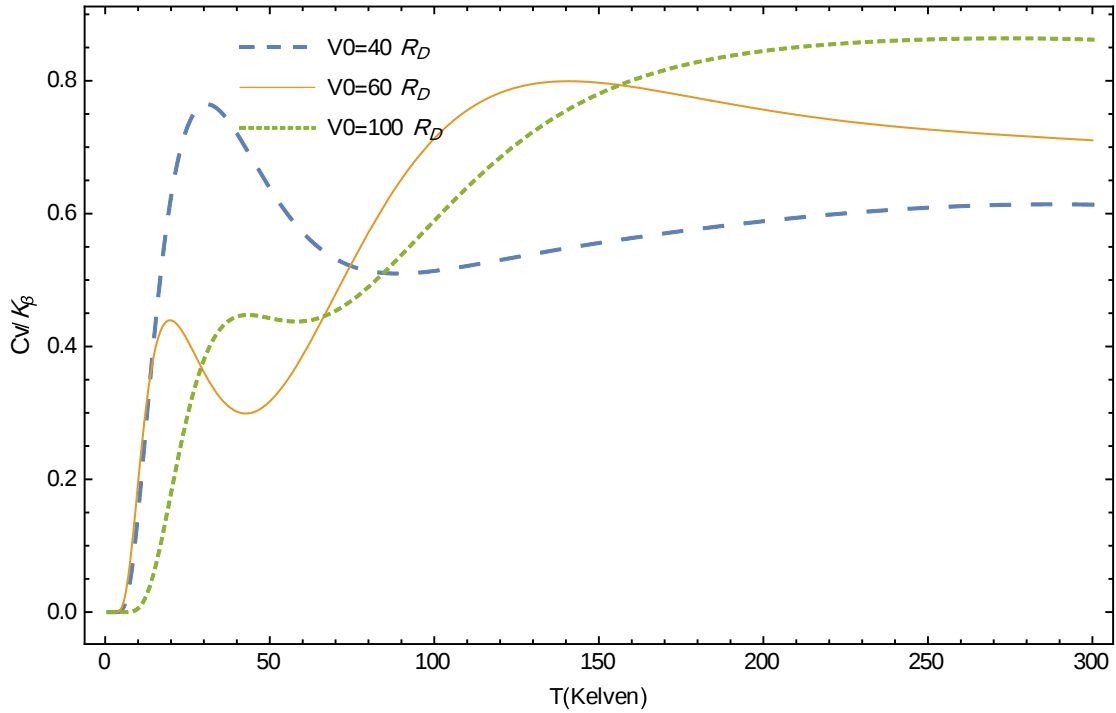
Figure (3-9): Heat Capacity of donor impurity QD ( C_v/K_B ) as function of temperature (T) for different values V_0 = 40R_D, 60R_D, 100R_D at constant R = 2a_D, N = 3D .
