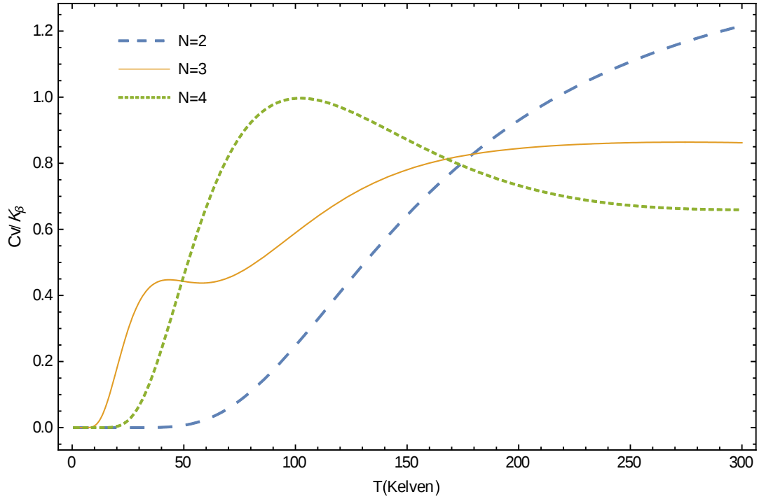
Figure (3-11): Heat Capacity of donor impurity QD ( C_v/K_\beta ) as function of temperature( T) for different values of N = 2D, 3D, 4D at constant V_0 = 100R_D , R = 2a_D .
