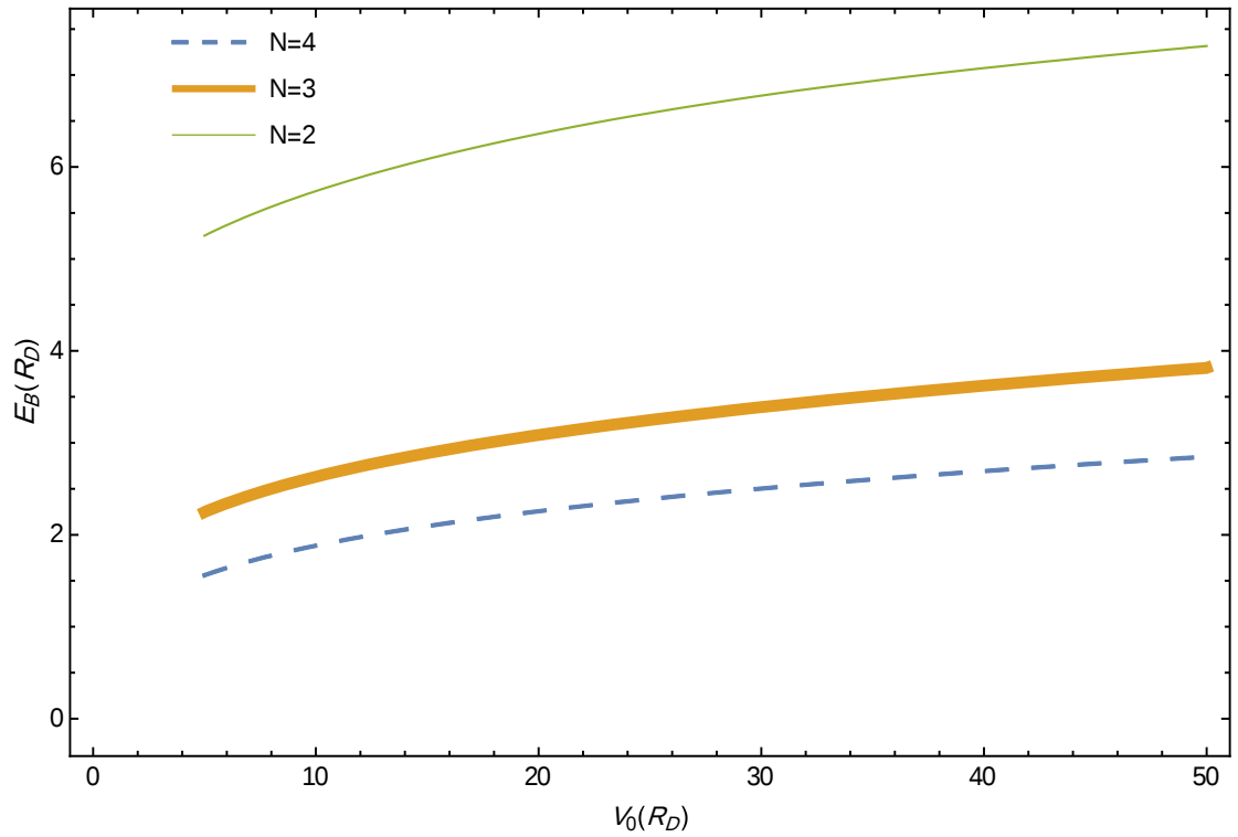
Figure (3- 5): Ground state binding donor energy E_B(1,0) as function of potential well depth ( V_0 ) and R = 2a_D for different values of dimension N = 2D, 3D, 4D .
