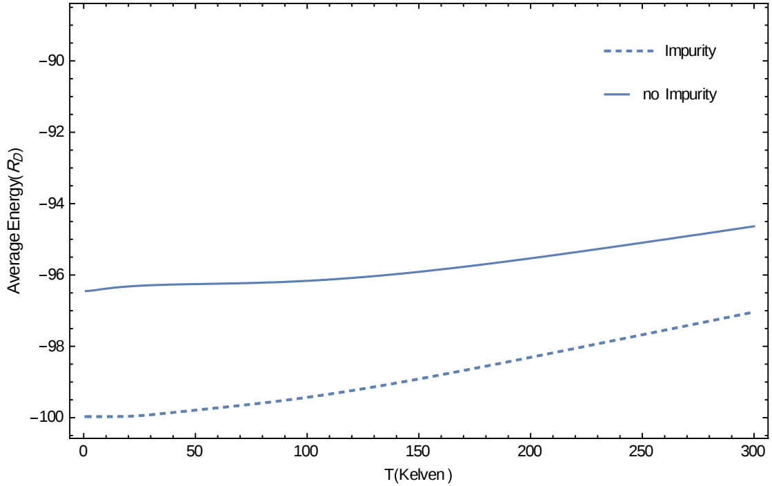
Figure (3-6): Average energy of QD as function of temperature (T) with donor impurity and without impurity at constant R = 2a_D , V_0 = 100R_D , N = 3D .
