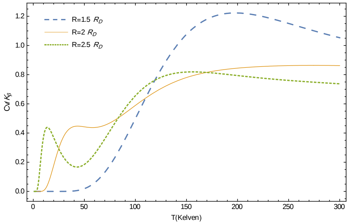
Figure (3-10): Heat Capacity of donor impurity QD ( C_v/K_B ) as function of temperature (T ) for different values of R = 1.5a_D, 2a_D, 2.5a_D at constant V_0 = 100R_D, N = 3D .
