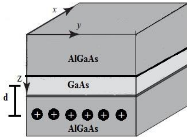
Figure (1-3): The structure of two-dimensional electron confined in GaAs layer bounded to an off donor impurity located in the AlGaAs layer.
