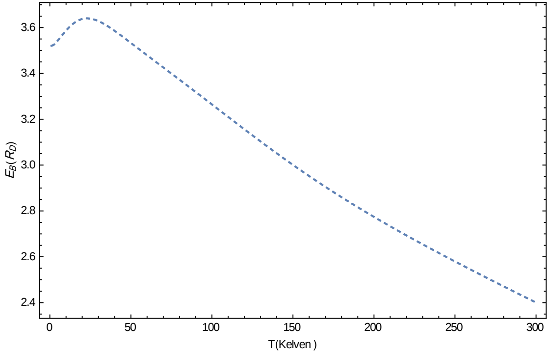
Figure (3-7): 3D Average binding energy of donor impurity in QD as function of temperature (T) at constant R = 2a_D , V_0 = 100R_D .
