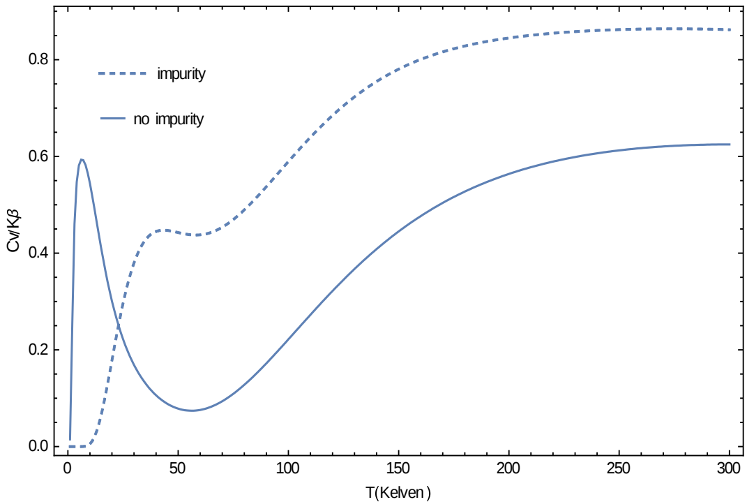
Figure (3-8): Heat Capacity of QD ( C_v/K_\beta ) as function of temperature (T ) with donor impurity and without impurity at constant R = 2a_D , V_0 = 100R_D , N = 3D
