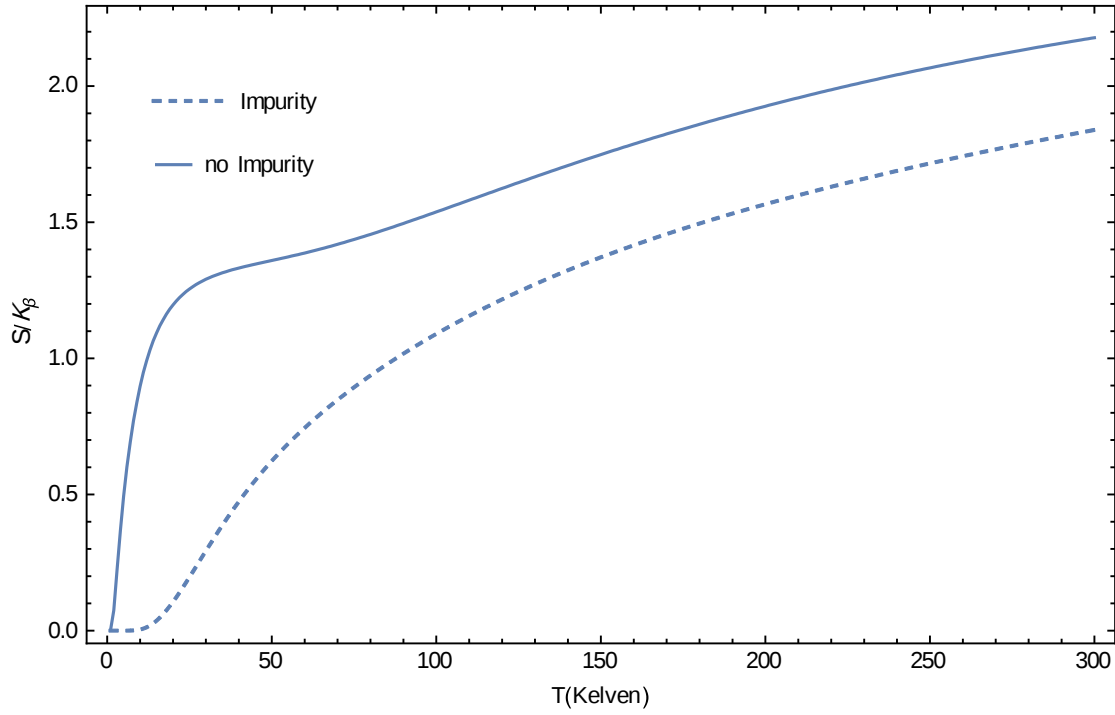
Figure (3-12): Entropy of QD ( S/K_B ) as function of temperature ( T ) with donor impurity and without impurity at constant R = 2a_D , V_0 = 50R_D , N = 3D .
