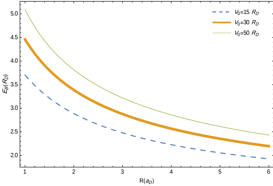
Figure (3-3): Ground state binding energy levels E_B(1,0) in QD as function of dot radius ( R ) for different values of V_0 = 15R_D, 30R_D, 50R_D , N = 3D .
