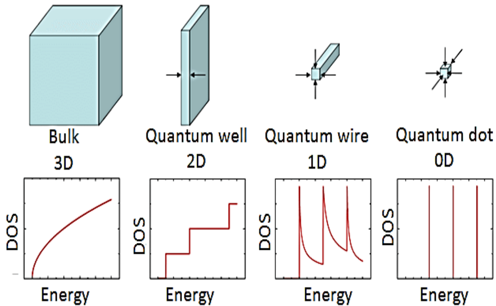
Figure (1-1): Quantum confinement in nanostructure and density of state as function of energy.
