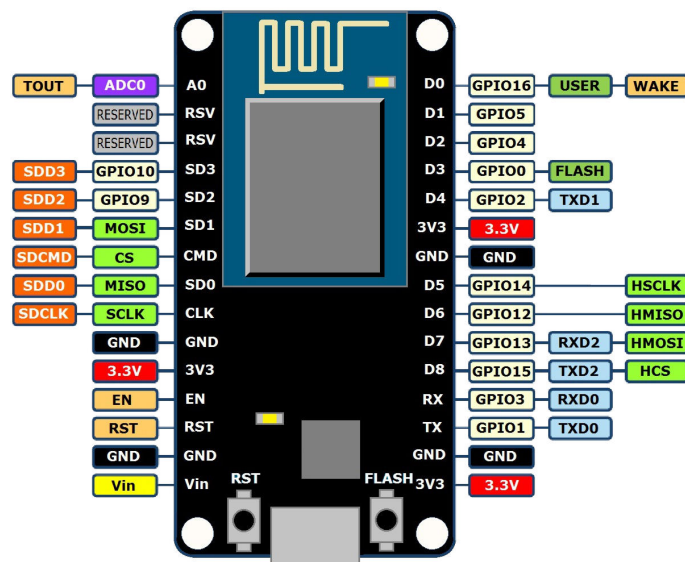
Figure 3: MCUNode ESP8266
