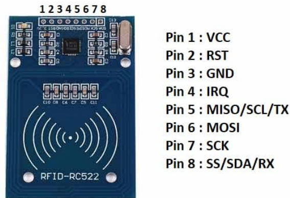
Figure 8: RFID reader
