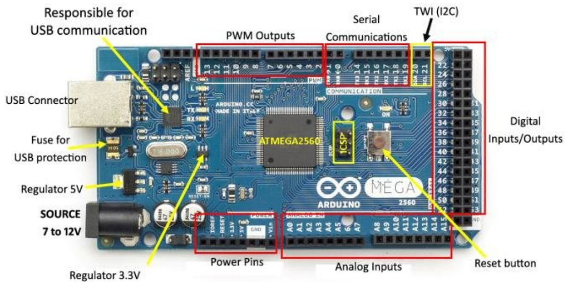
Figure 1: Arduino Mega 2560
