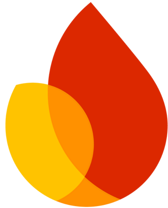
FIREBASE (NOTIFICATIONS)
