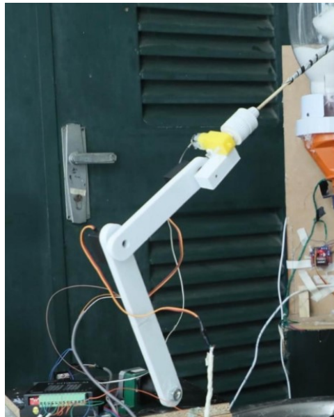
Figure 24: Arm structure.
