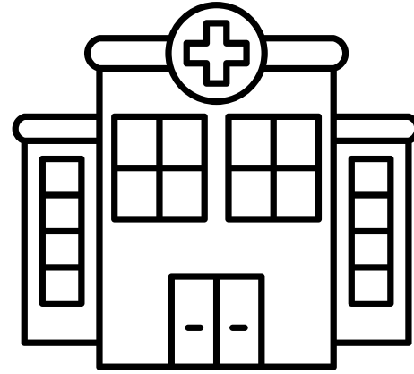
• Clinic Model
