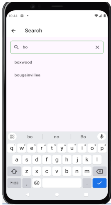
Figure 27:search suggestion
