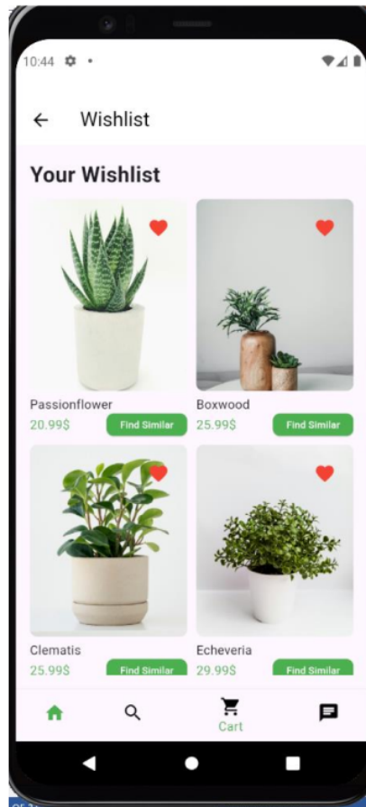
Figure 41:wishlist screen
