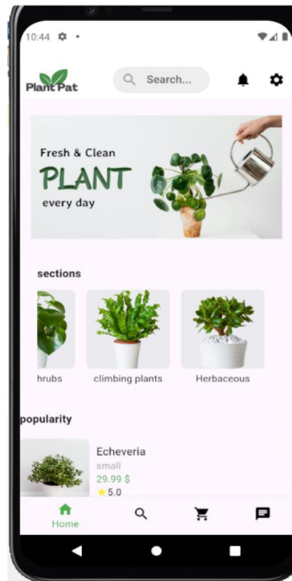
Figure19 :home screen
