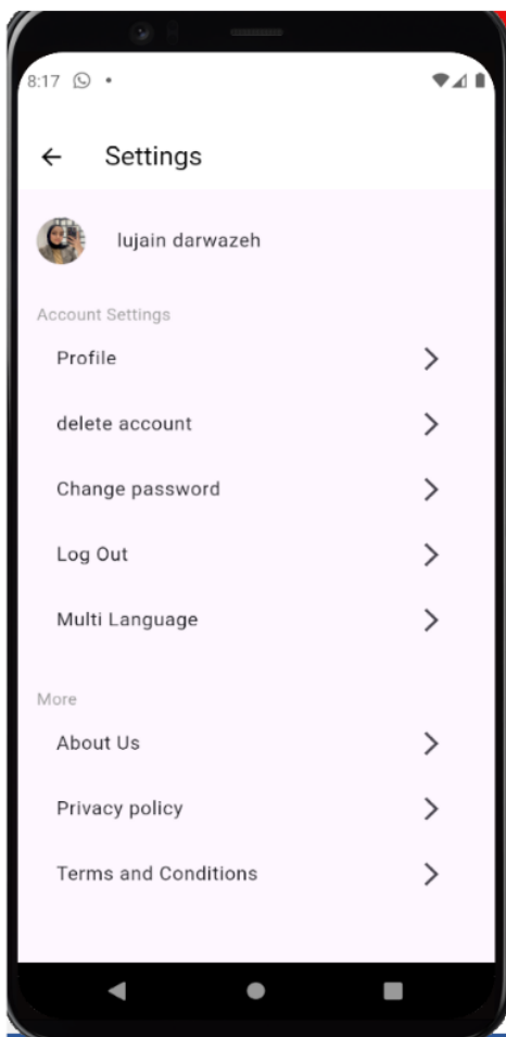
Figure 67:settings screen
