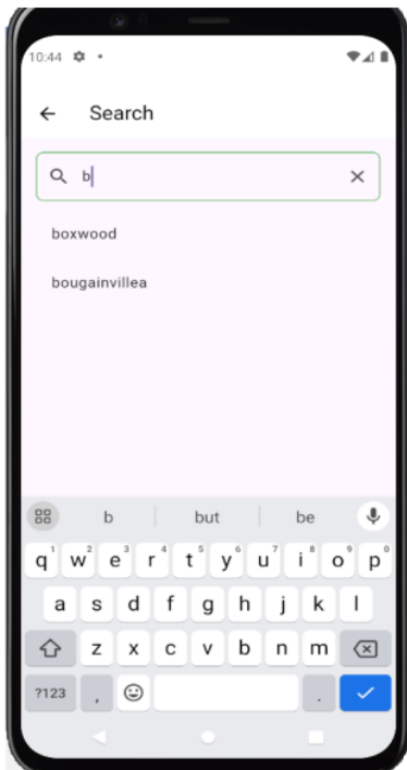
Figure 26:search suggestion
