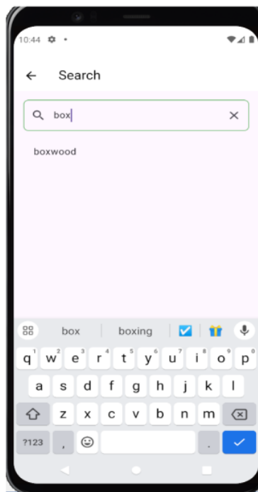
Figure 28:search suggestion
