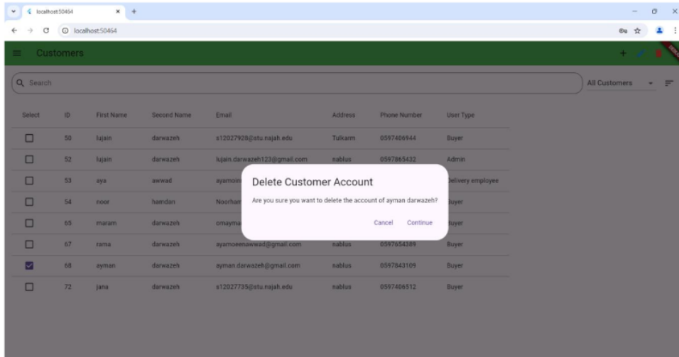
Figure 108:delete customer
