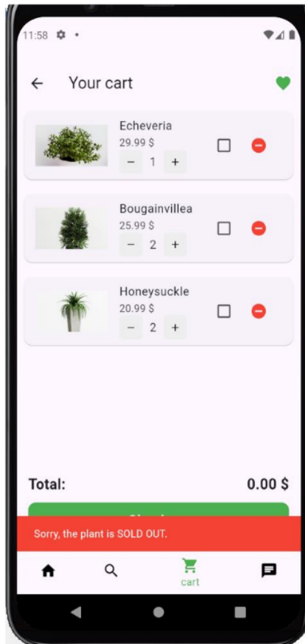
Figure 37: SOLD OUT
