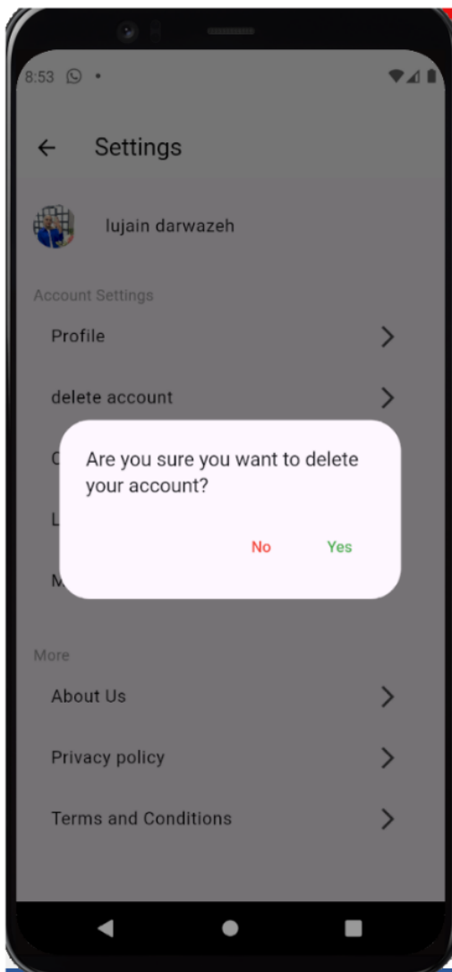
Figure 71:delete account
