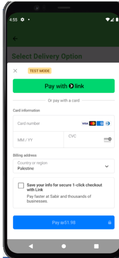
Figure 61:visa screen
