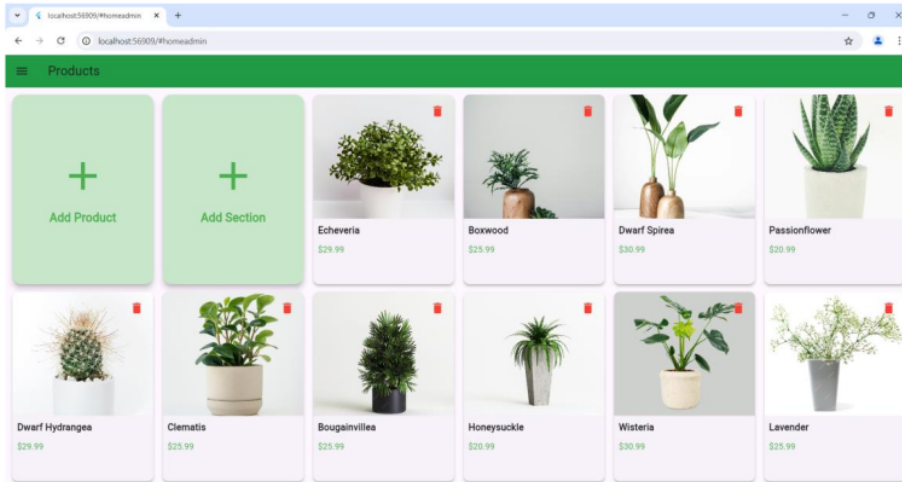
Figure 114:products screen
