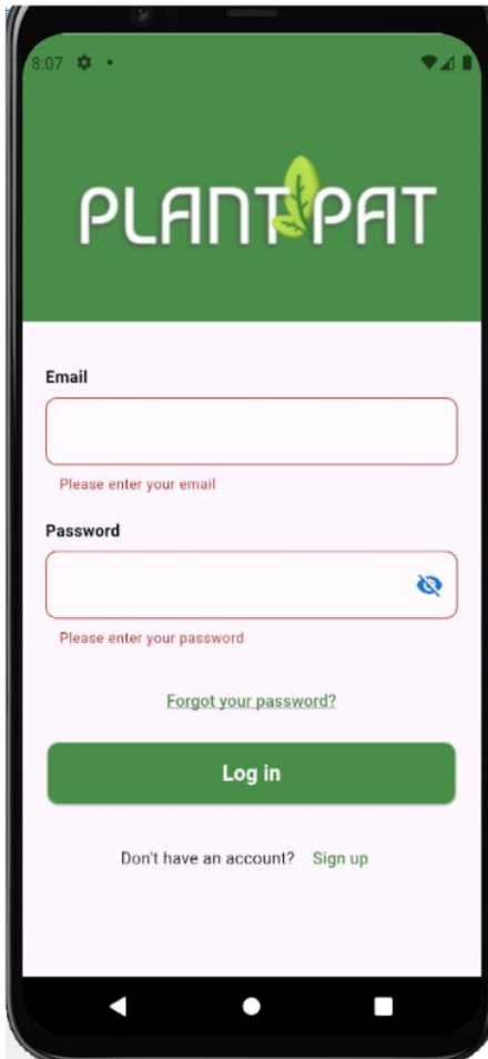
Figure10 :empty field
