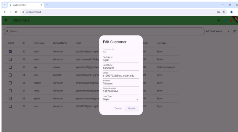
Figure 107:edit customer
