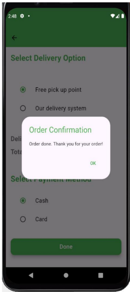
Figure 52:order confirmation
