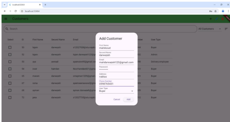
Figure 109: Add customer
