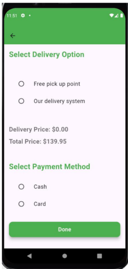
Figure 49:option screen
