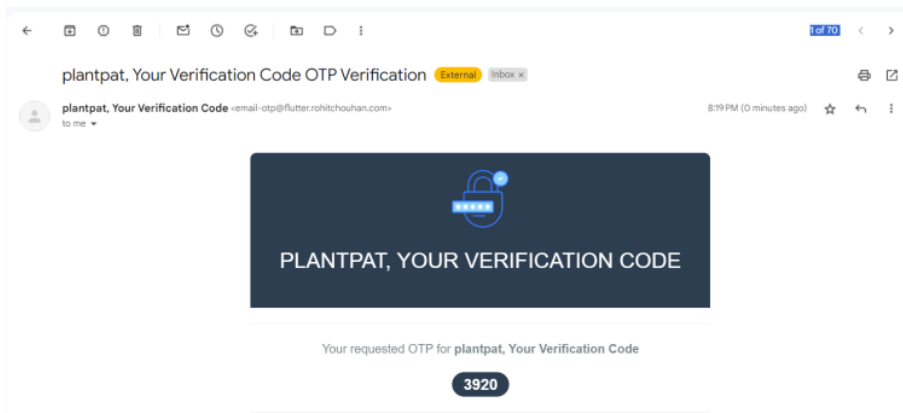
Figure 14:Verification code
