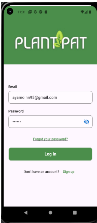
Figure 80:login delivery
