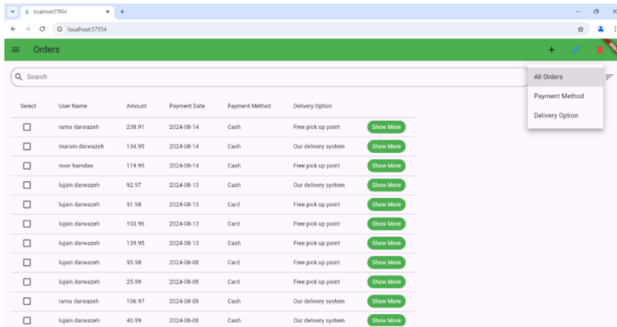
Figure 94:filter orders
