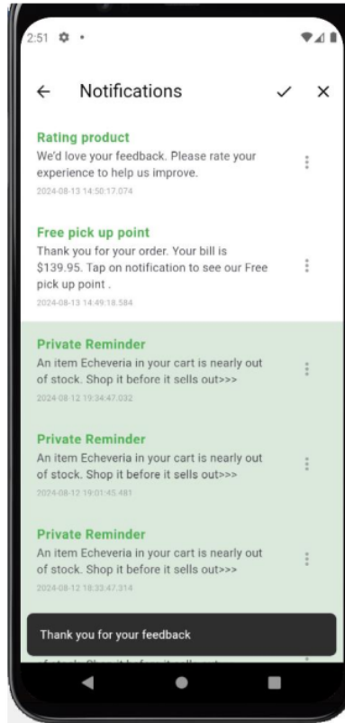
Figure59 :after submit
