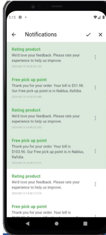
Figure 63: notification user
