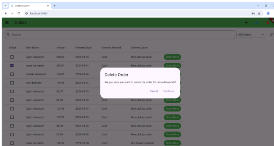
Figure 103:delete order
