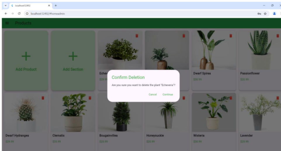
Figure 128:delete plant
