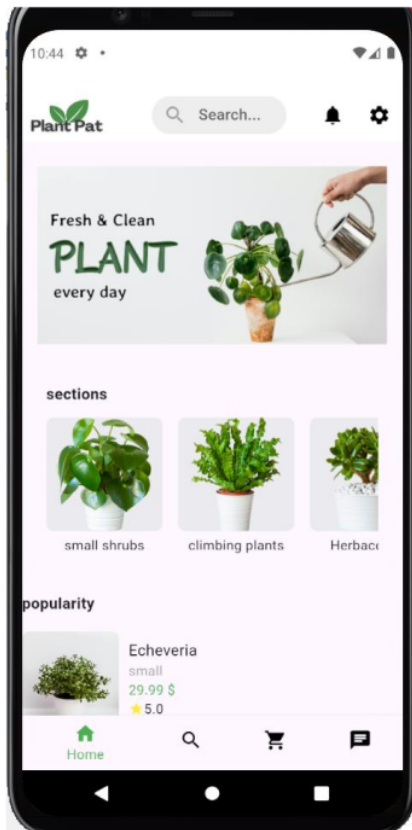
Figure 18:home screen
