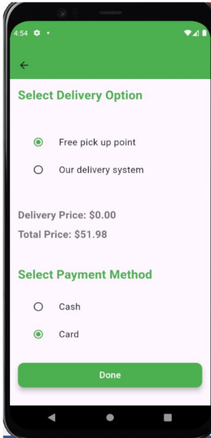
Figure 60:card option
