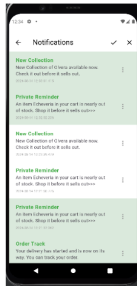
Figure 79:notifications screen
