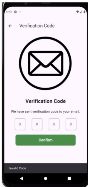
Figure 15:invalid code
