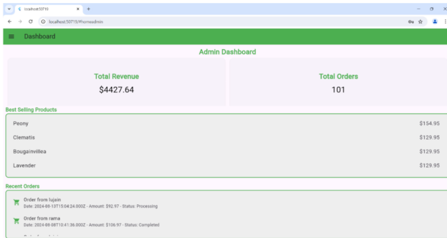
Figure 91:Dashboard screen
