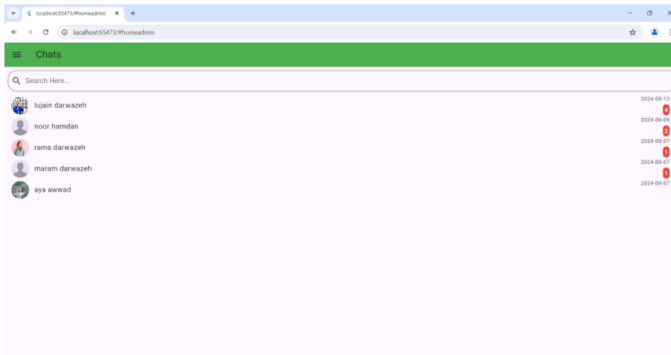
Figure 111:chat screen
