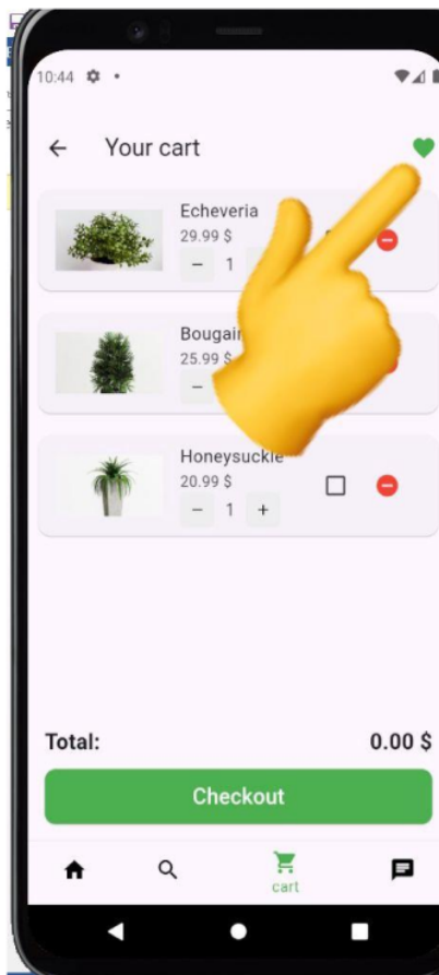
Figure 40:wishlist icon
