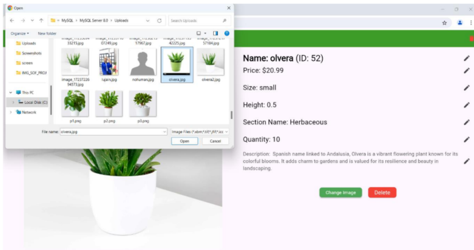
Figure 126:change image
