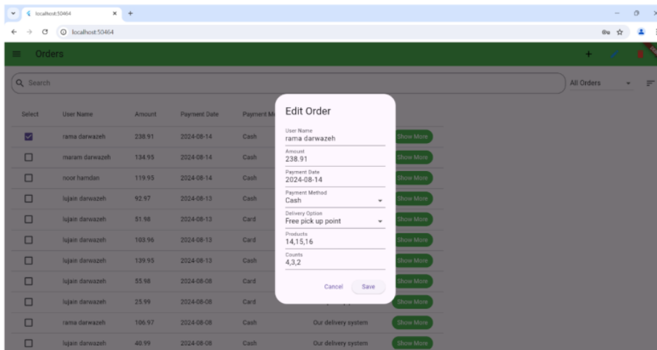
Figure 97:edit order
